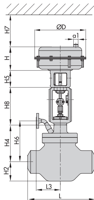
Type 3281-7 with welding ends
