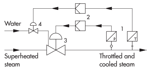
Fig. 1: Type 3281-1 Pneumatic Steam Conditioning Valve
