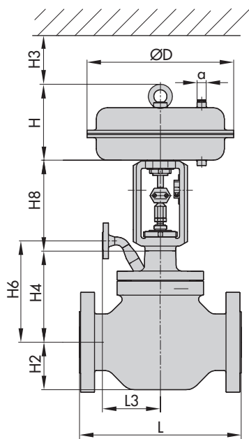
Type 3281-1 with flanges
