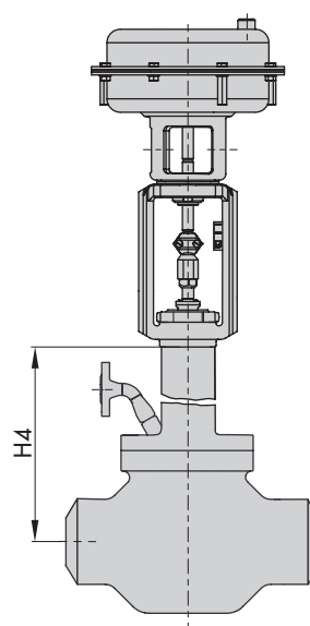
Type 3281-7 with insulating section and welding ends
