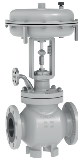
Fig. 1: Type 3281-1 Pneumatic Steam Conditioning Valve
