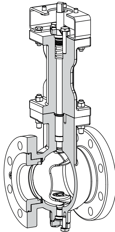
Fig. 4: Insulating section for Type 3310 Segmented Ball Valve
