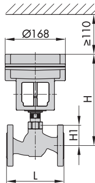
Type 3213/2780-2: DN 15 to 50
