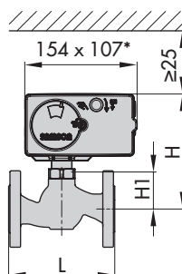
Type 3213/5827: DN 15 to 50 * Dimensions for actuators with double stroking speed: 154x140
