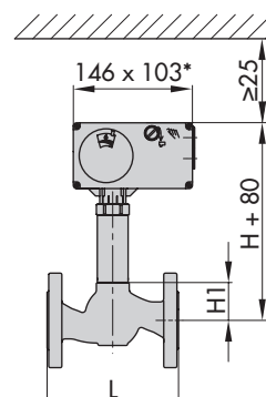
Version for steam Type 3213/5724-3: DN 15 to 50 Type 3213/5724-8: DN 15 to 50 * Dimensions for TROVIS 5724-3x3 Actuators: 146x136
