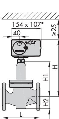
Type 3214/5827: DN 15 to 50 * Dimensions for actuators with double stroking speed: 154x140
