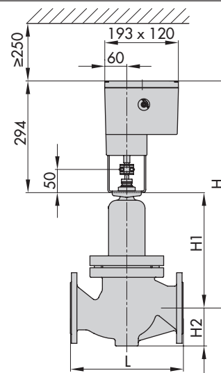
Type 3214/3374-11: DN 65 to 100
