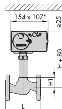
Version for steam Type 3213/5827: DN 15 to 50 * Dimensions for actuators with double stroking speed: 154x140
