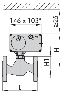
Type 3213/5724-3: DN 15 to 50 Type 3213/5724-8: DN 15 to 50 * Dimensions for TROVIS 5724-3x3 Actuators: 146x136
