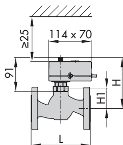
Type 3213/5857: DN 15 to 25 Type 3213/5757-3: DN 15 to 25 Type 3213/5757-7: DN 15 to 25
