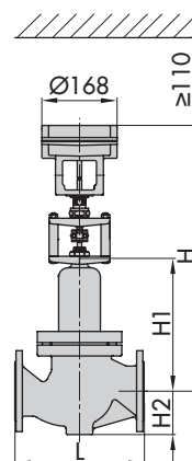
Type 3214/2780-2: DN 65 to 100
